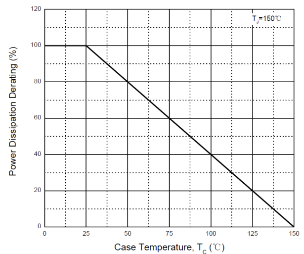
Fig.12 - Power Derating
