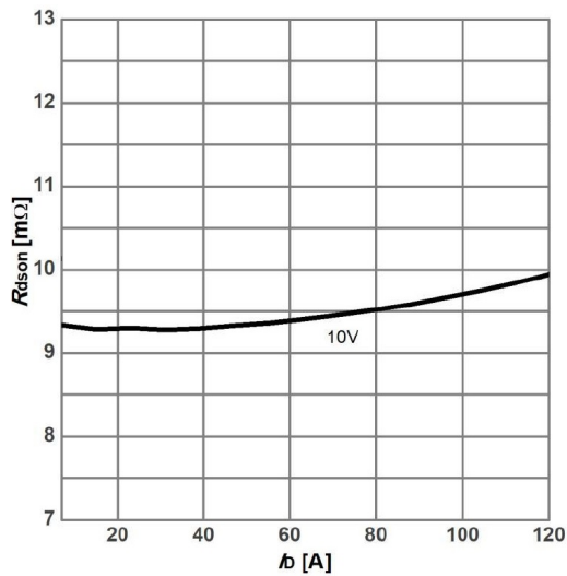
Fig.5 - Drain-Source On-Resistance
