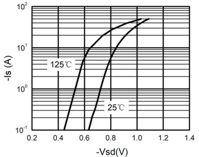
Fig.6 - Forward Characteristic
