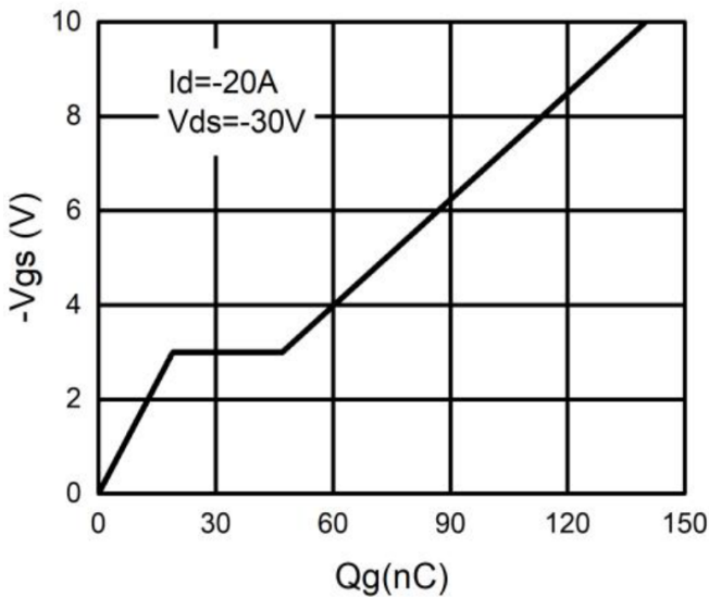
Fig.5 - Gate charge
