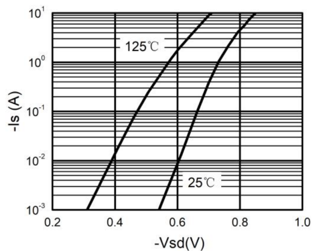
Fig.6 - Forward Characteristic
