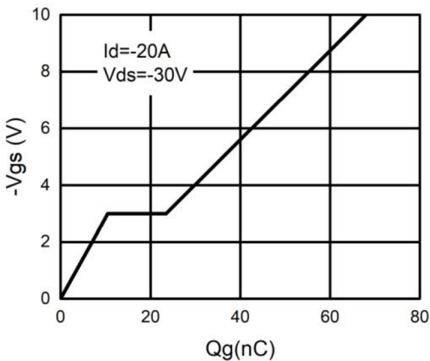
Fig.5 - Gate charge
